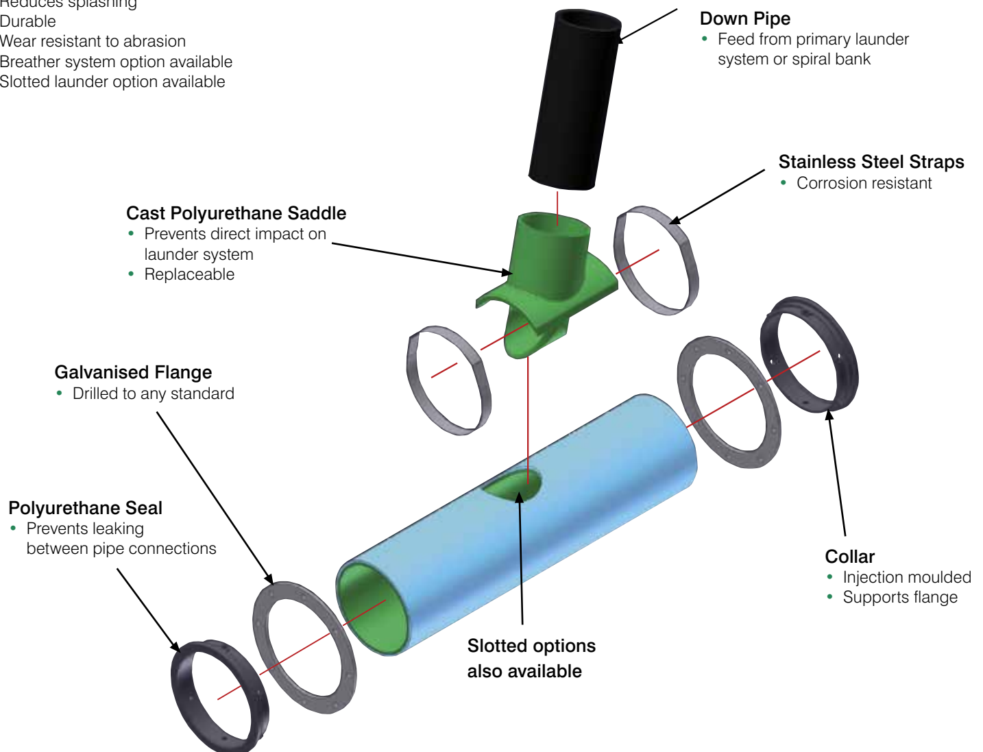
uPVC Lined Pipe Launder
